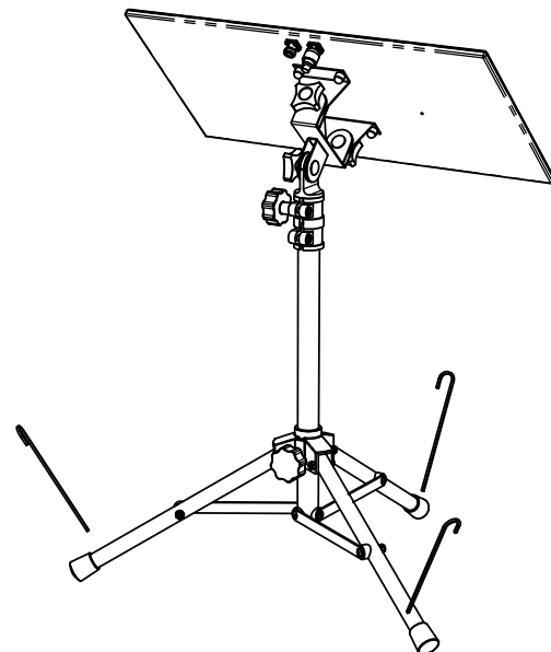
PICTORIAL VIEW (SHOWN MOUNTED TO 056A BRACKET ASSEMBLY & 1096B ANTENNA)
