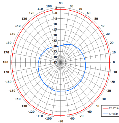
Azimuth Pattern
